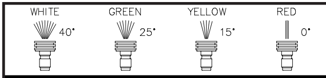
Figure 8 – Spray patterns of nozzles
