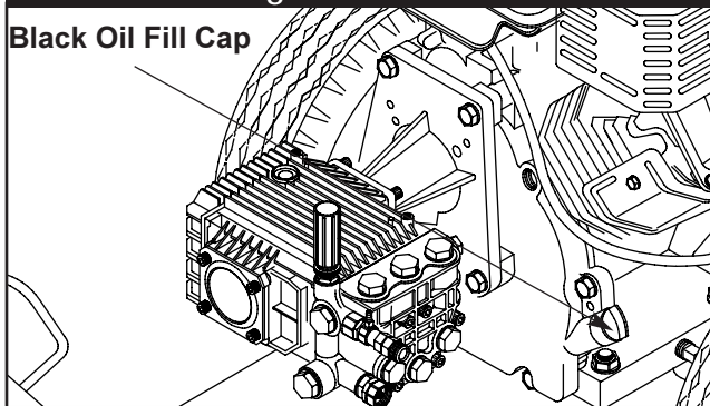
Figure 2 — Add oil to engine crankcase. Do not attempt to start engine without adding oil.
