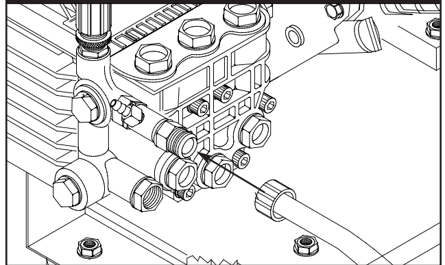
Figure 5 — Connect high pressure hose to pump.
