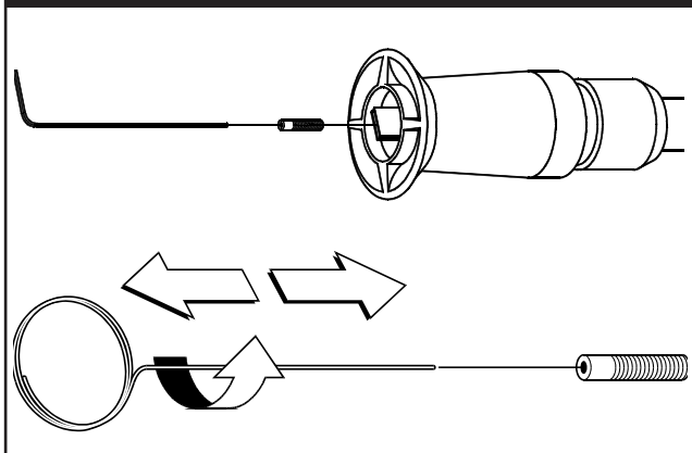
Figure 17 – Removing and cleaning nozzle.
