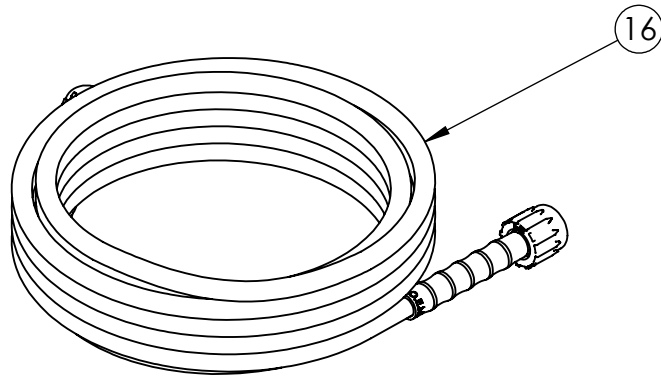
HOSE, MORFLEX 1/4" X 25' X 3100PSI M22(M) X M22(F) PART NO. 7106419
