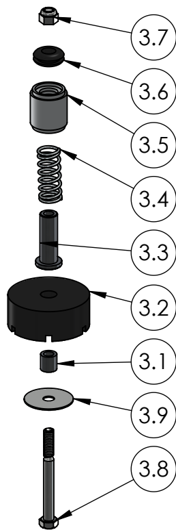
FOOT KIT, WS SERIES SPRING PART NO. 7106951
