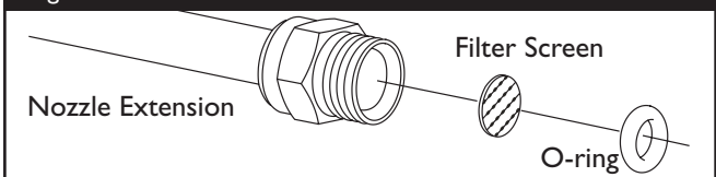
Figure 18 — Clean In-Line Filter
