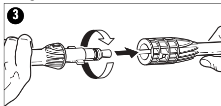
Figure 4 - Connect the high pressure hose (H1) to the water (OUTLET) (A) on the cleaner by first inserting the brass end of the hose into the threaded brass outlet, then snugly threading on the coupling.
