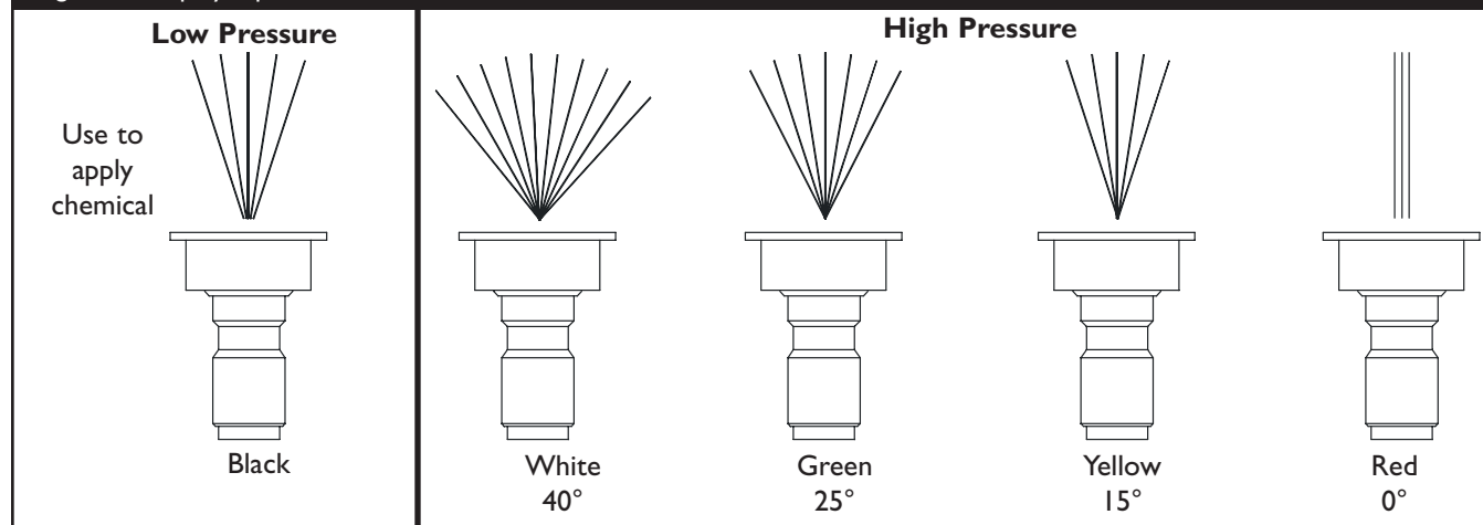
Figure 7 — Spray Tips
