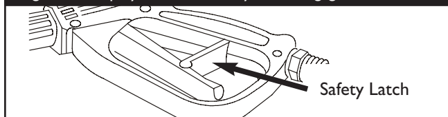
Figure 6 — Spray Gun with Safety Latch Engaged
