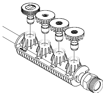
Figure 13 — Install Spray Tips in Holder
