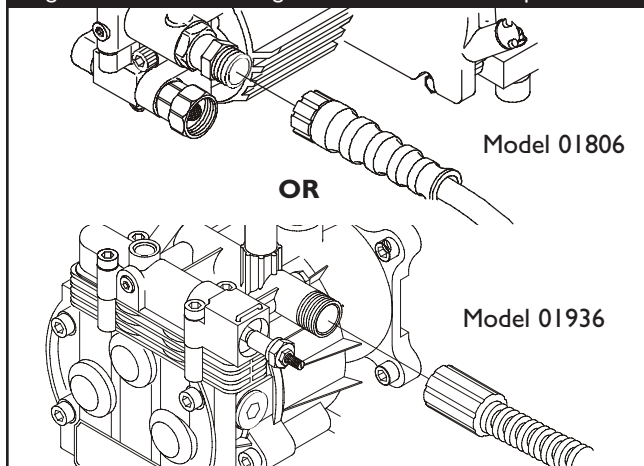
Figure 11 — Connect High Pressure Hose to Pump
