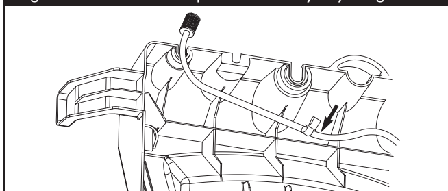
Figure 6 — Slide Metal Clip onto Accessory Tray Flange
