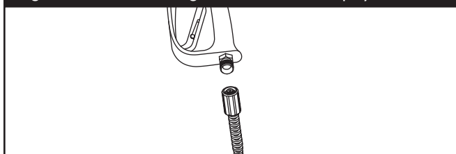
Figure 10 — Connect High Pressure Hose to Spray Gun
