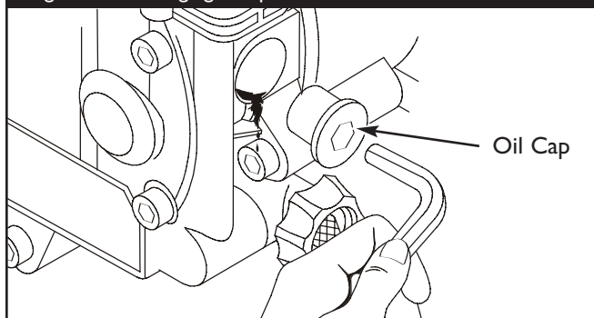
Figure 19 - Changing Pump Oil
