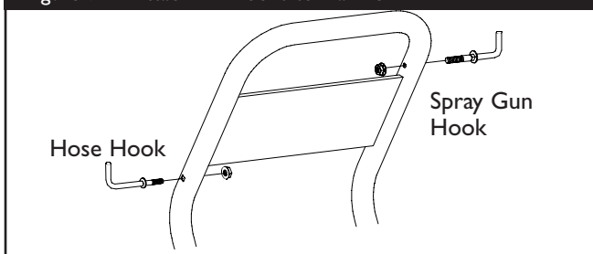
Figure 9 — Attach "L" Hooks to Handle
