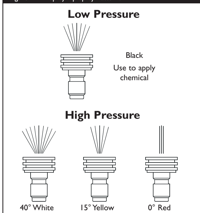
Figure 14 — Spray Tip Spray Patterns
