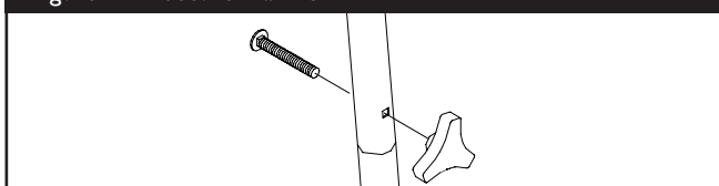
Figure 2 — Secure Handle
