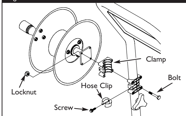
Figure 7 — Install Hose Reel on Handle
