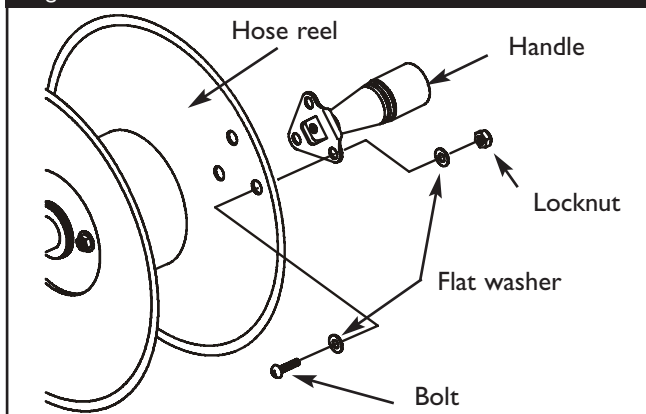
Figure 6 — Attach Handle to Reel
