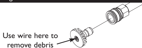
Figure 10 — Nozzle Maintenance
