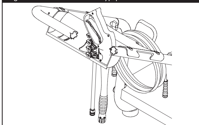
Figure 35 — Porte-accessoires typique
