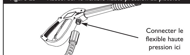
Figure 25 — Raccorder le flexible haute pression au pistolet
