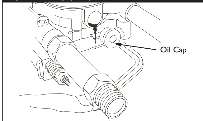
Figure 21 - Changing Pump Oil
