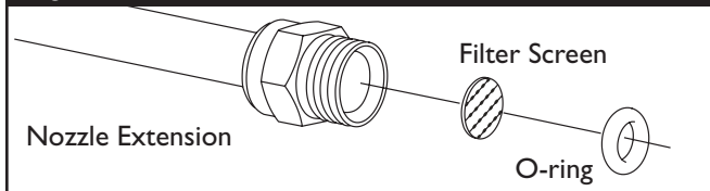
Figure 18 — Clean In-Line Filter
