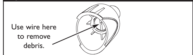
Figure 19 — Nozzle Maintenance
