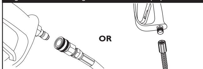
Figure 7 — Connect High Pressure Hose to Spray Gun
