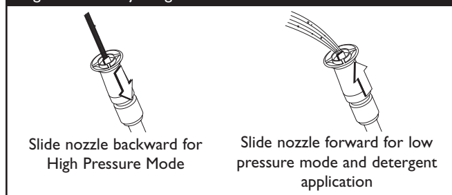
Figure 12 — Adjusting Nozzle for Pressure
