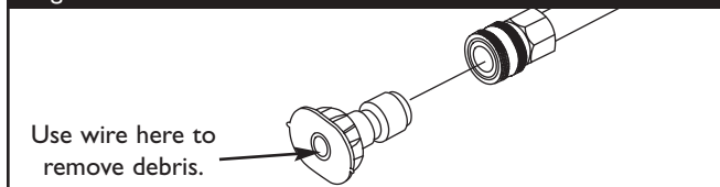
Figure 19 — Nozzle Maintenance
