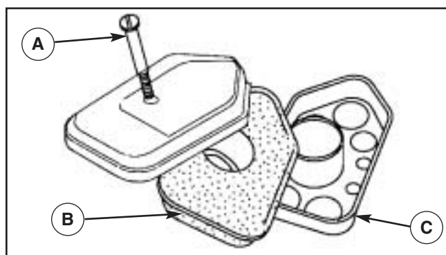
Figure 21: Air cleaner
