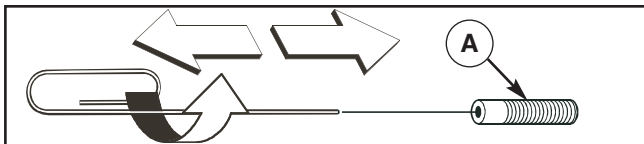
Figure 18: Cleaning orifice
