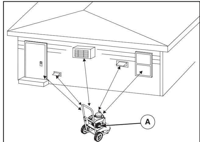
Figure 7: Pressure washer clearance for typical pressure washer
