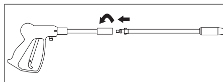
Figure 4 - Gun/Lance Connection
