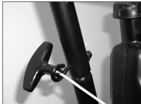
Figure 2 -Secure engine pull cord
