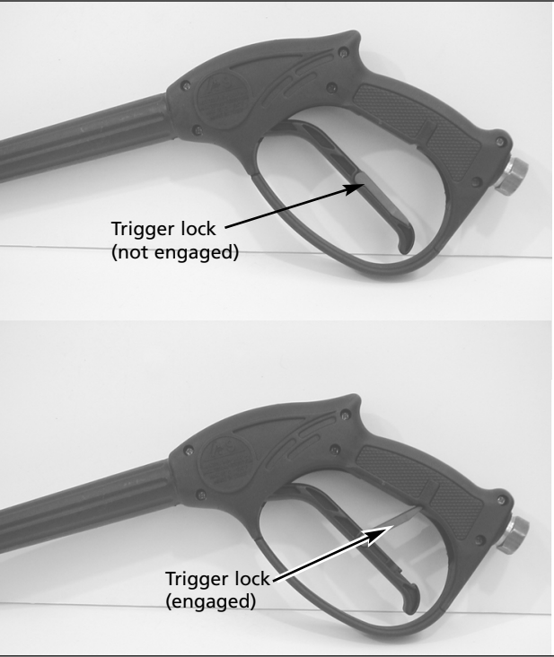
Figure 11 - Trigger lock
