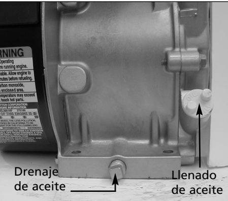
Figure 22 - Oil drain and fill locations
