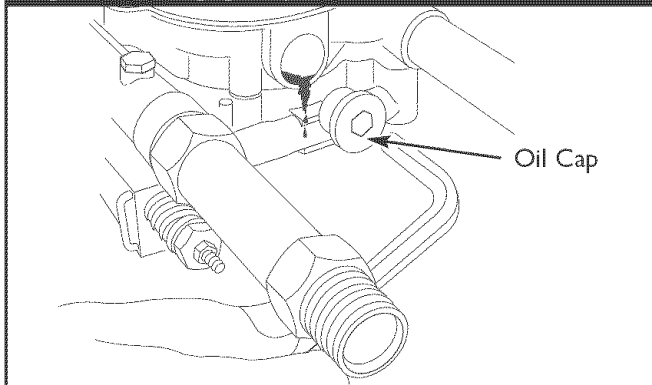
Figure 16 - Changing Pump Oil
