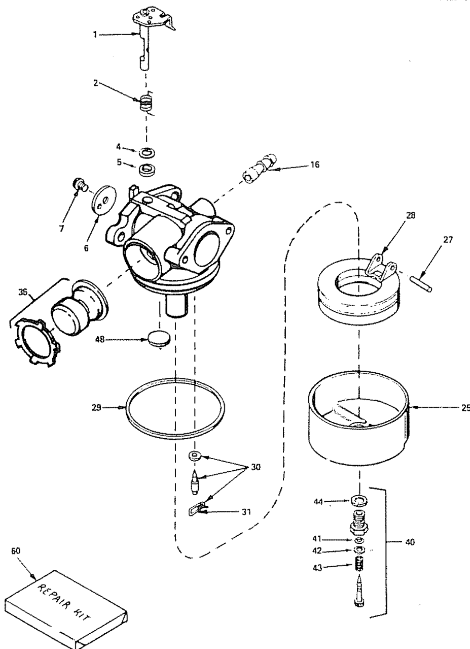
Carburetor No. 632589
