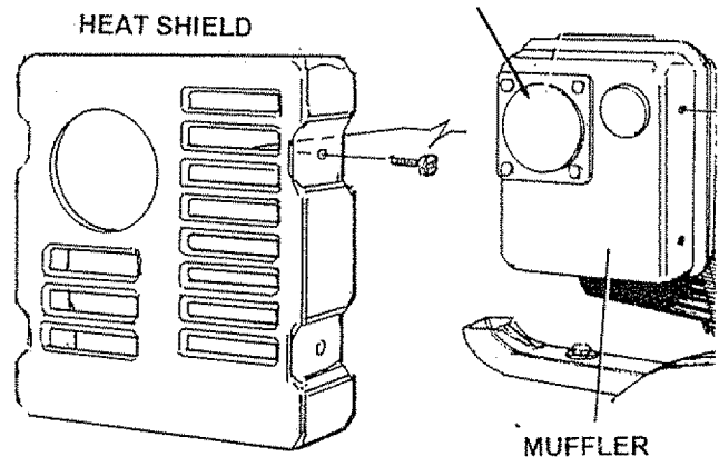
SPARK ARRESTOR SCREEN (P/N 83083)
