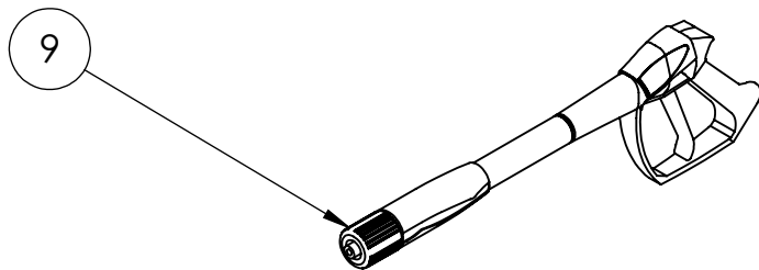
GUN, 3000PSI M22(M) INLET, M22(F) OUTLET PART NO. 7104847
