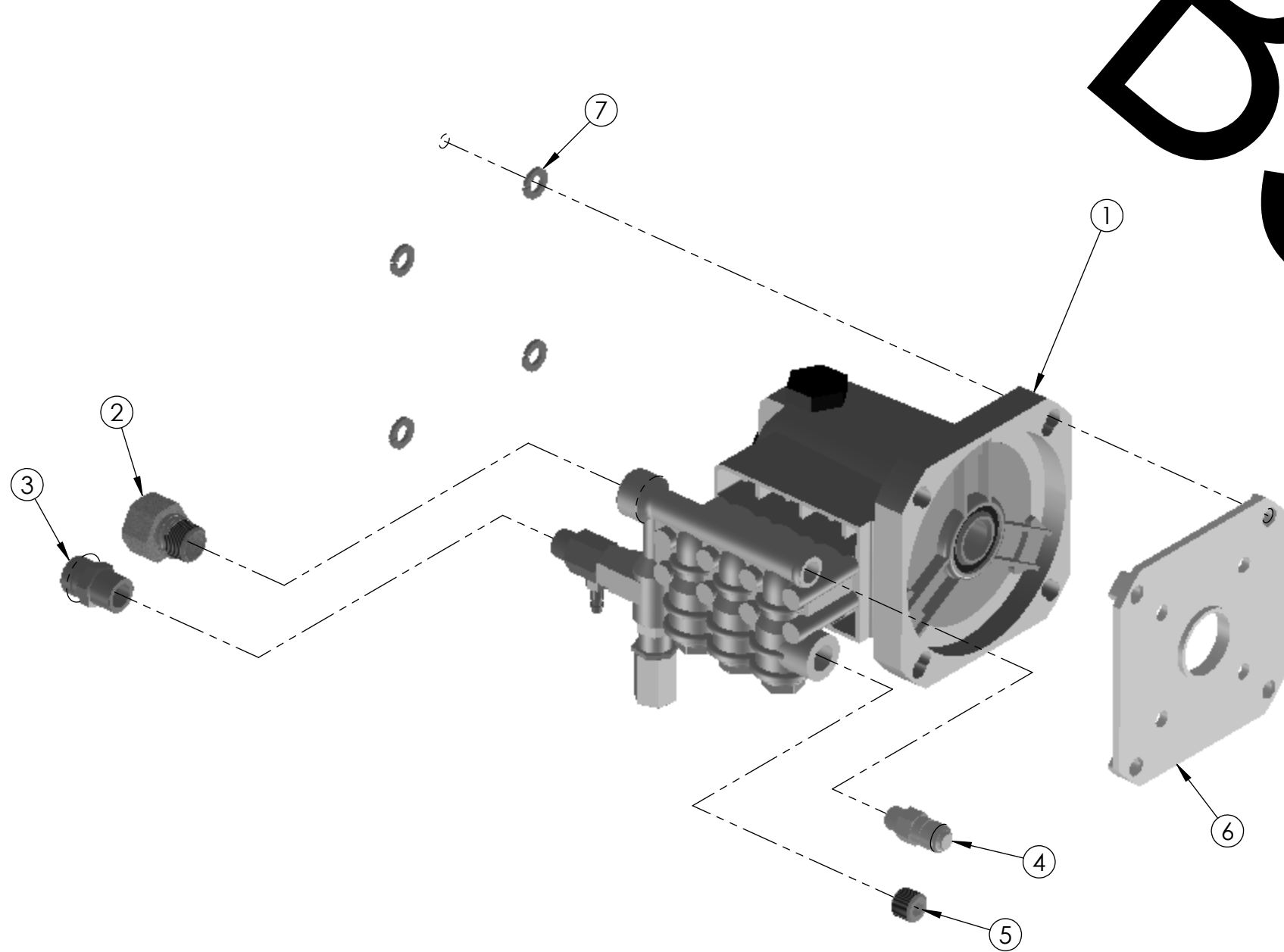
PUMP, HORIZONTAL SERVICE KIT PART NO. 7105023
