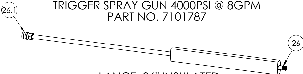
LANCE, 36" INSULATED PART NO. 7100550
