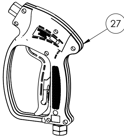
SPRAY GUN 5000PSI @ 10GPM PART NO. 7100393
