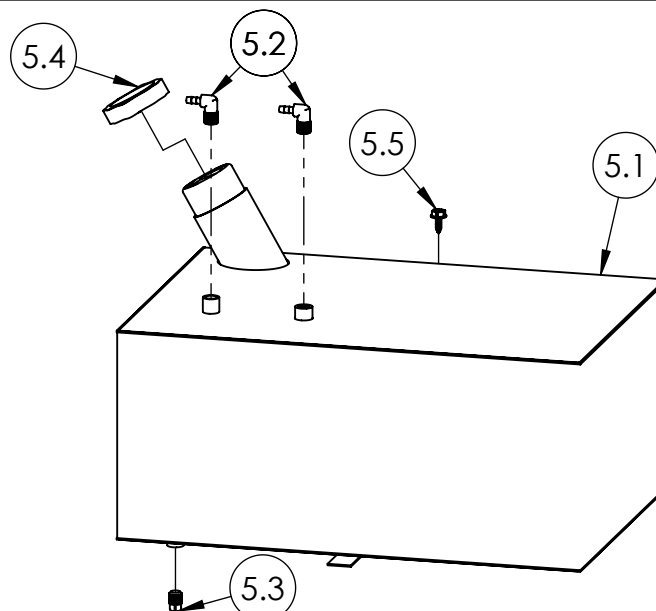
GAS TANK, SVC ASSY DEWALT COBALT PART NO. 7106197
