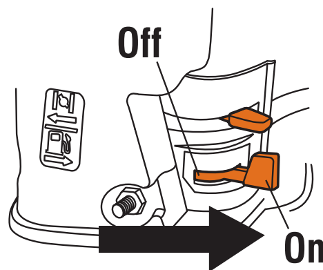
Figure 20 – Fuel Valve
