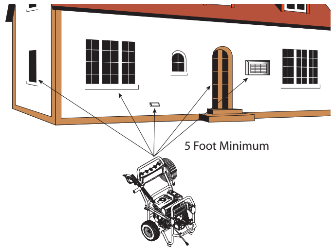
Figure 19 – Building Clearances
