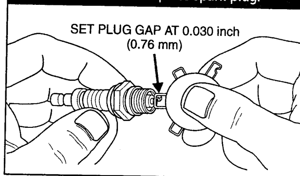
FIGURE 17 — Replace spark plug.
