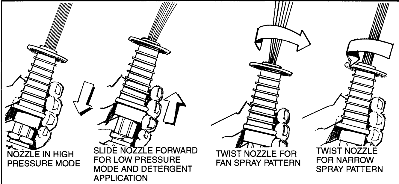
FIGURE 13 — Using the Adjustable Nozzle
