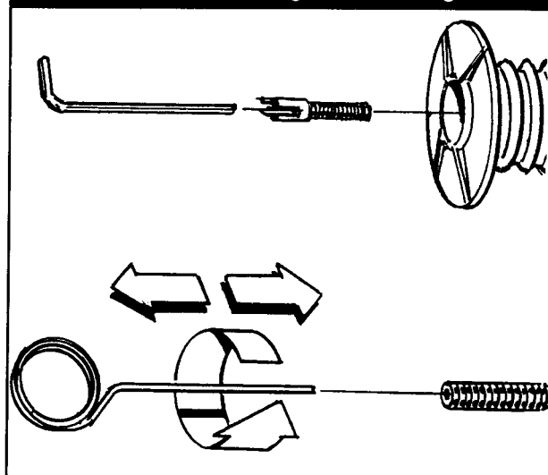
FIGURE 19 — Removing and Cleaning Nozzle
