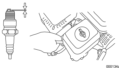
Figure 4-8. Spark Plug
