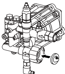
Figure 2-8. Inspect Inlet Screen
