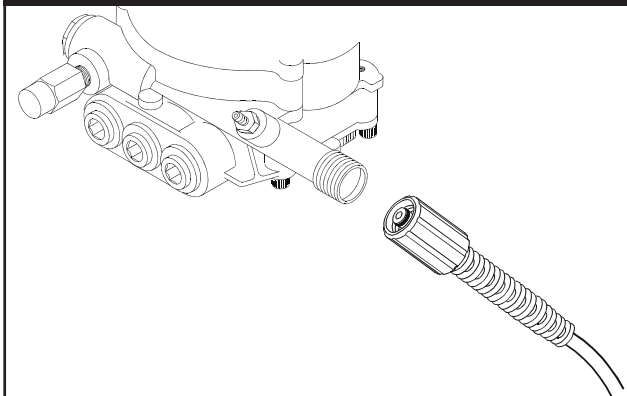
Figure 5 — Connect high pressure hose to pump.
