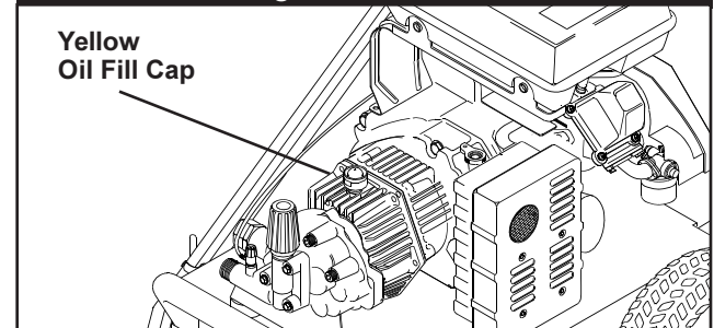
Figure 4 — Add oil to engine crankcase. Do not attempt to start engine without adding oil.
