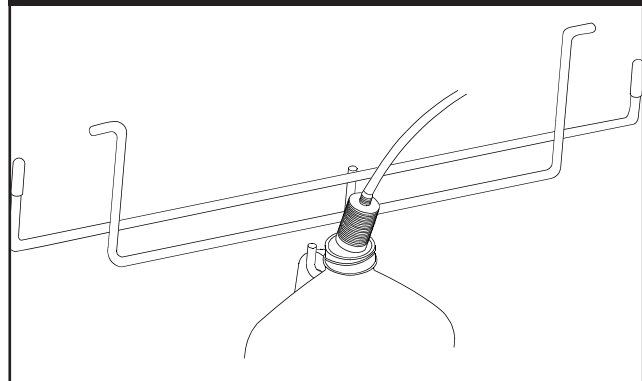
Figure 12 — Insert the small filter into container of cleaning solution.
