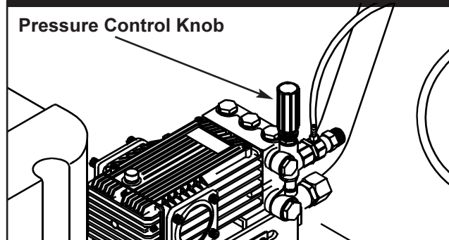
Figure 10 – Pressure control knob.
