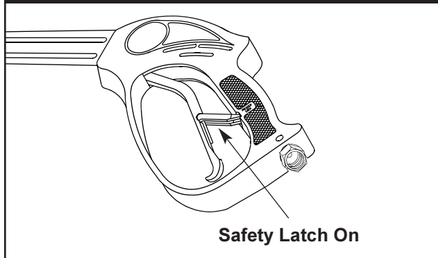
Figure 10 – Safety Latch.
