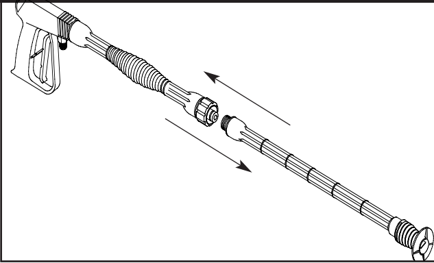
Figure 9 — Connect nozzle extension to spray gun.
