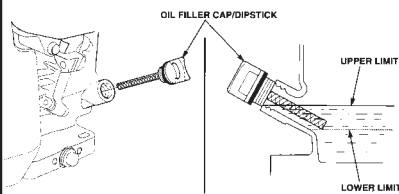
Figure 3 — Add oil to engine crankcase. Do not attempt to start engine without adding oil.
