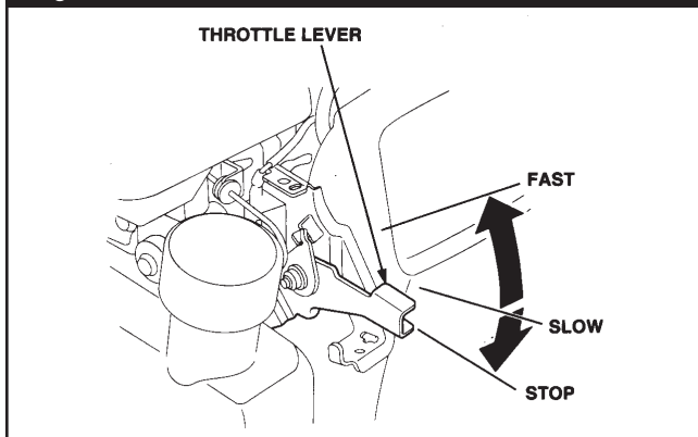
Figure 11 — Throttle Lever
