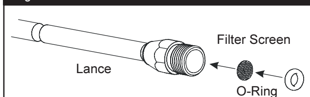
Figure 16 — Service In-Line Filter
