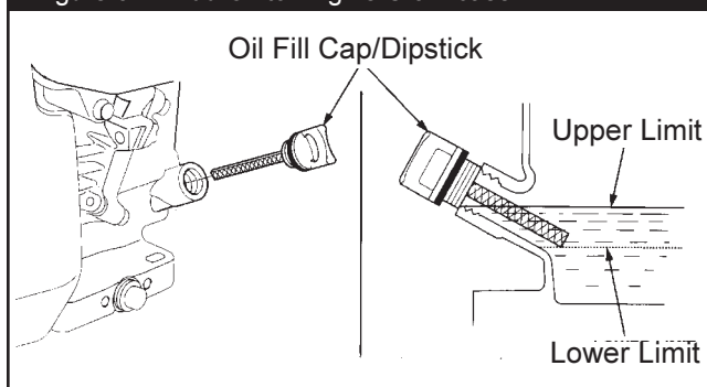
Figure 3 — Add Oil to Engine Crankcase
