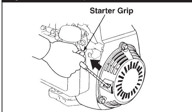
Figure 12 — Starter Grip
