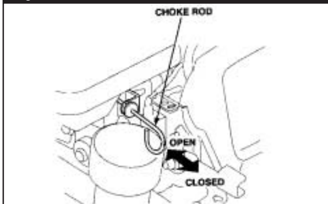
Figure 10 — Choke Rod
