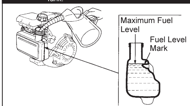
Figure 4 — Add Regular Unleaded Gasoline to Fuel Tank.
