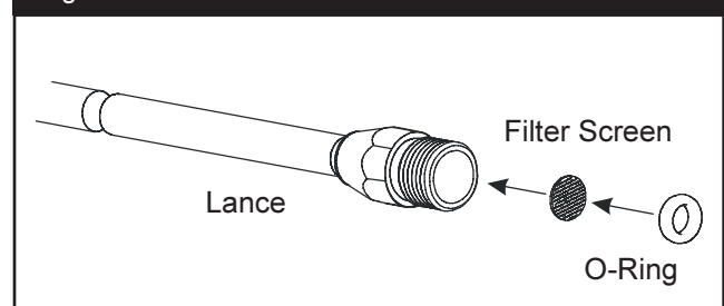
Figure 16 — Service In-Line Filter
