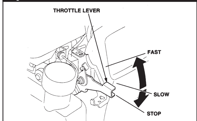
Figure 10 — Throttle Lever
