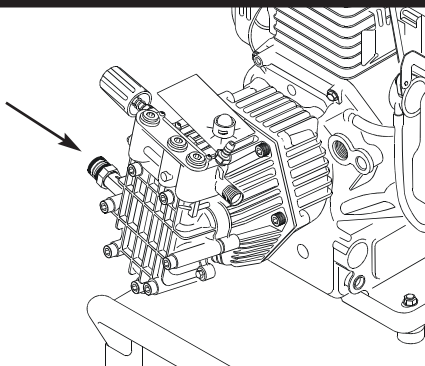
Figure 7 — Connect the Garden Hose to Water Inlet and Turn ON the Water.
