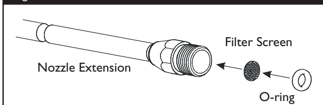
Figure 13 — Clean In-Line Filter
