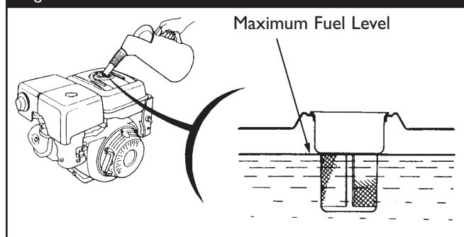
Figure 2 — Add Gasoline to Fuel Tank
