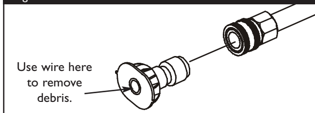
Figure 14 — Nozzle Maintenance
