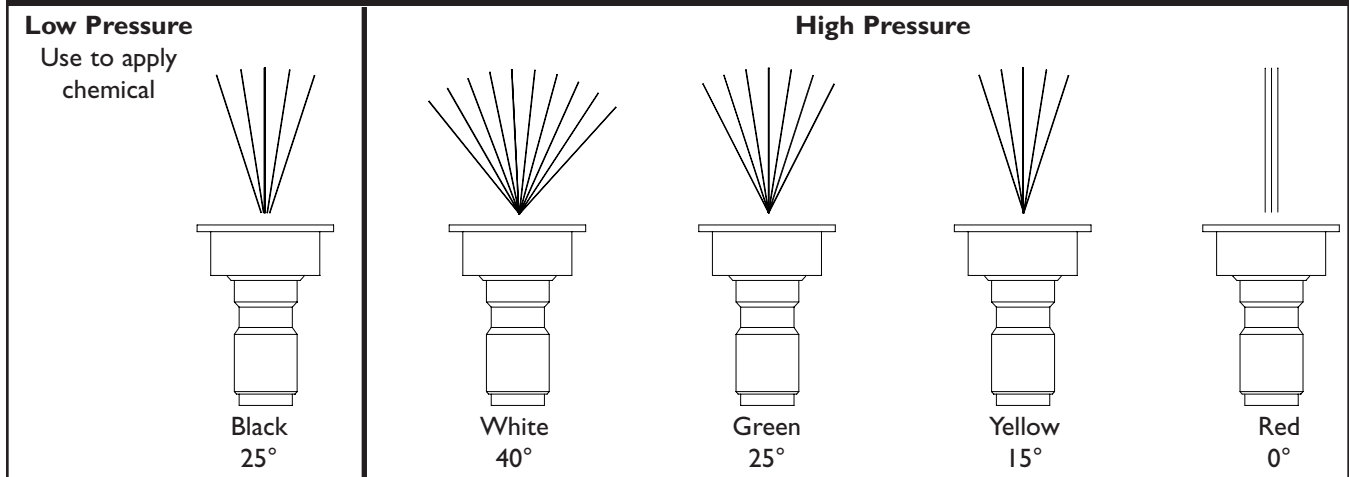
Figure 11 — Nozzles
