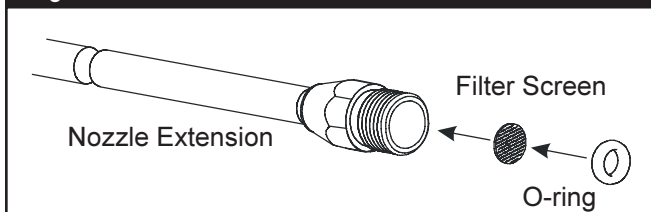
Figure 14 — Clean In-Line Filter
