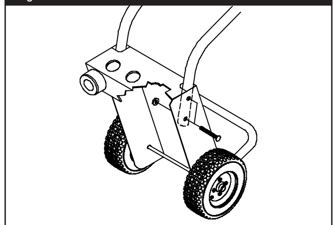
Figure 1 — Attach Handle to Pressure Washer
