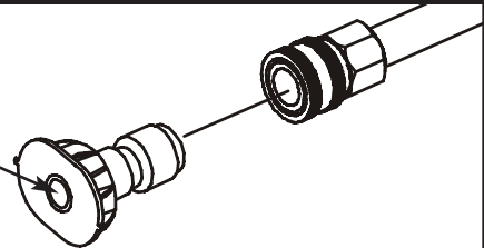
Figure 14 — Nozzle Maintenance
