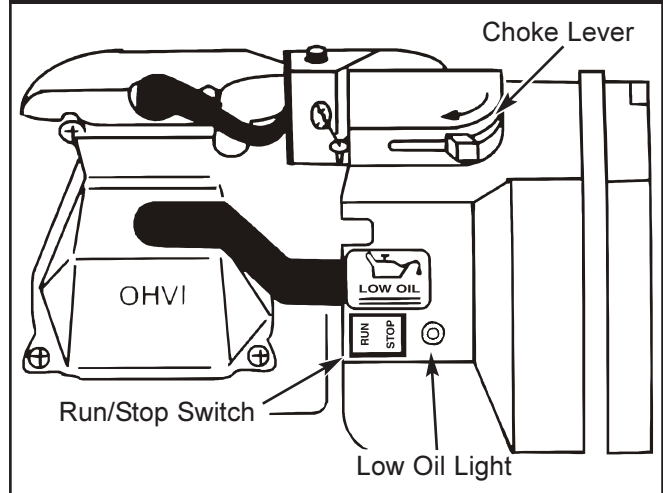
Figure 10 — Engine Controls
