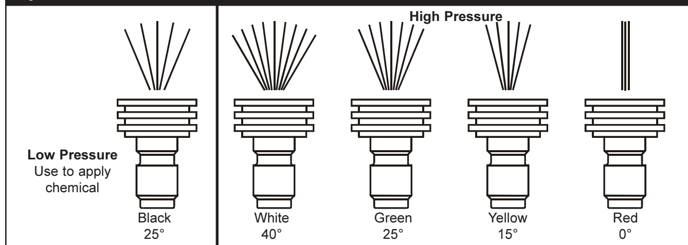
Figure 11 — Quick Connect Nozzles
