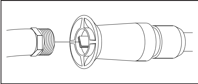
Figure 16 — Backflushing the Nozzle
