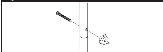
Figure 2 — Secure Handle.
