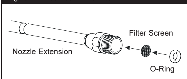
Figure 17 — Service In-Line Filter
