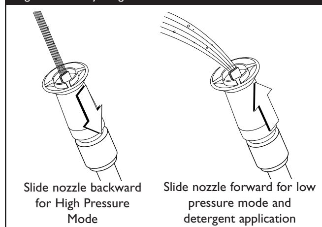
Figure 11 — Adjusting Nozzle for Pressure
