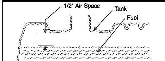
Figure 6 — Add Gasoline to Fuel Tank
