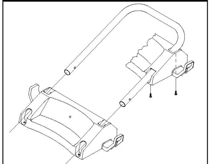
Figure 1 — Attach Accessory Tray
