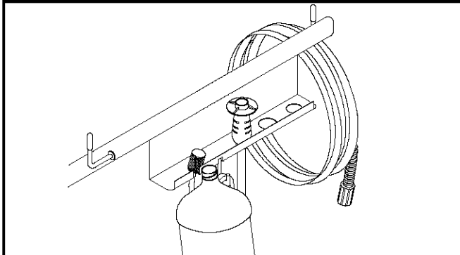
Figure 15 — Typical Accessory Tray
