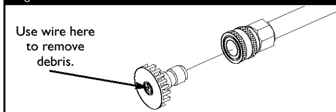
Figure 9 — Nozzle Maintenance
