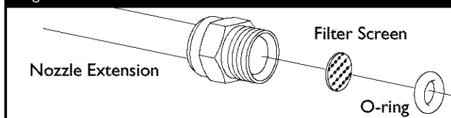
Figure 8 — Clean In-Line Filter
