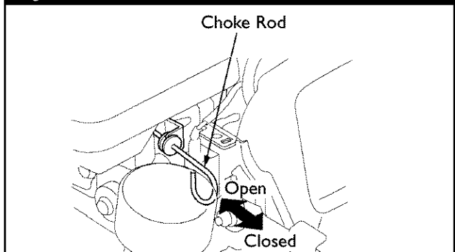
Figure 14 — Choke Positions
