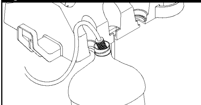
Figure 18 — Insert Filter into Container
