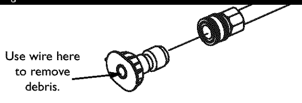
Figure 20 — Nozzle Maintenance
