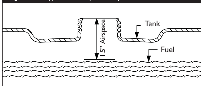
Figure 7 — Typical Fuel Expansion Space
