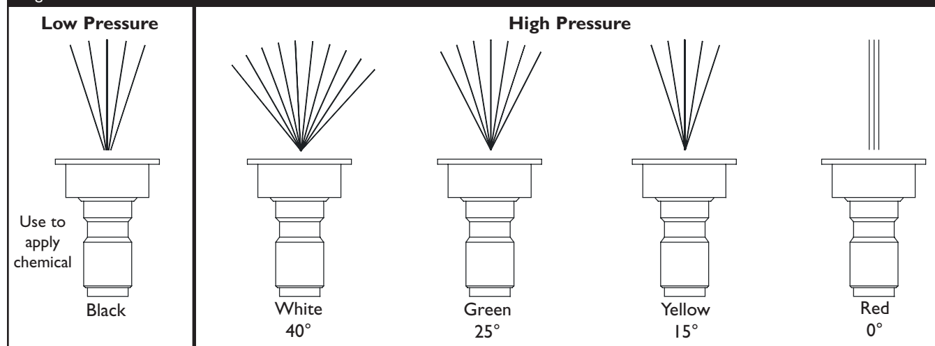
Figure 17 — Nozzles
